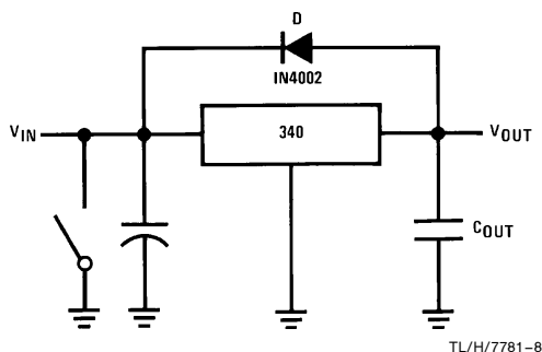
FIGURE 1. Input Short
