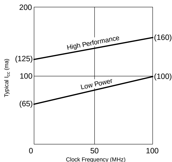
Figure 1: Typical I_{CC} vs. Frequency for XC9572
