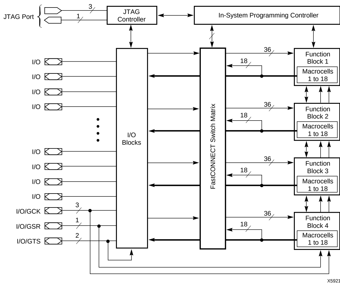
Figure 2: XC9572 Architecture
