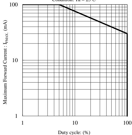
Max. Forward Current vs. Duty Cycle
