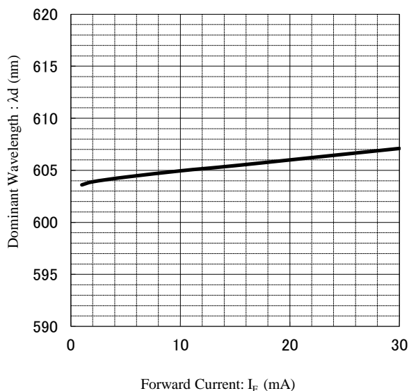
Forward Current vs. Dominant Wavelength
