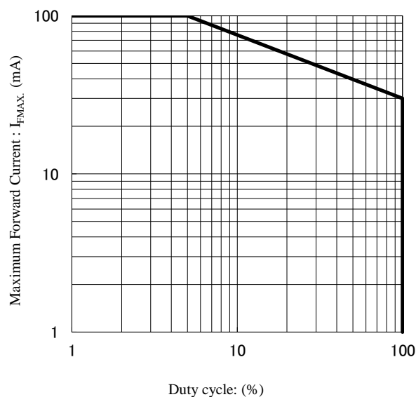
Max. Forward Current vs. Duty Cycle
