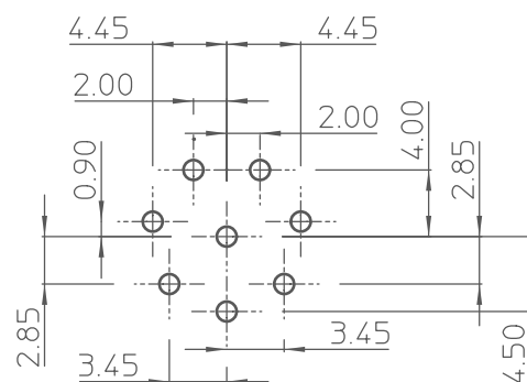
DRILLING PATTERN
