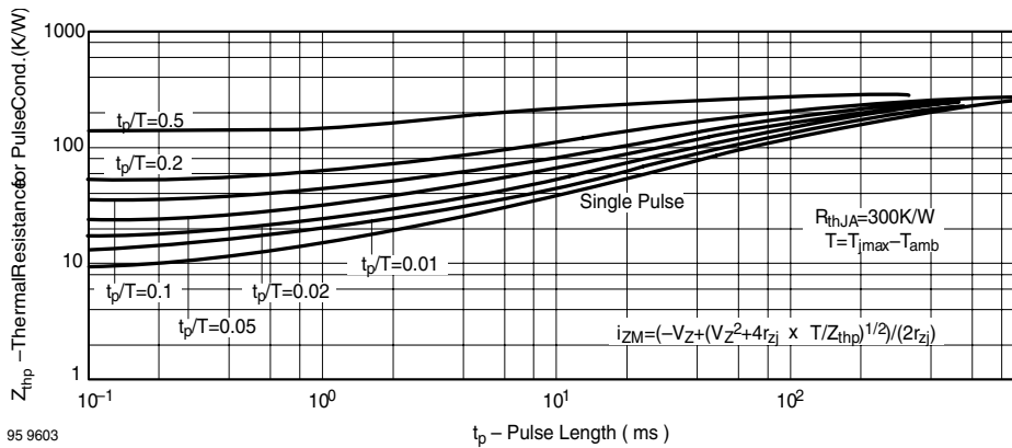
Fig. 10 Thermal Response
