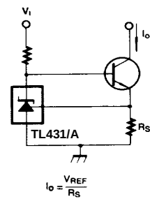
Figure 14. Constant-Current Sink
