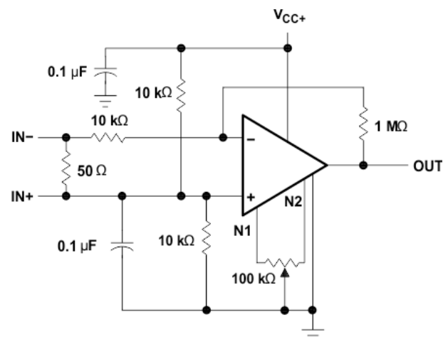
Figure 9-9. AC Amplifier
