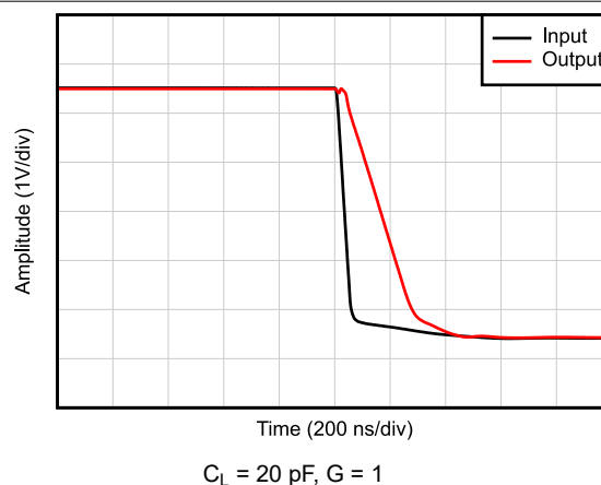
Figure 6-34. Large-Signal Step Response (Falling)
