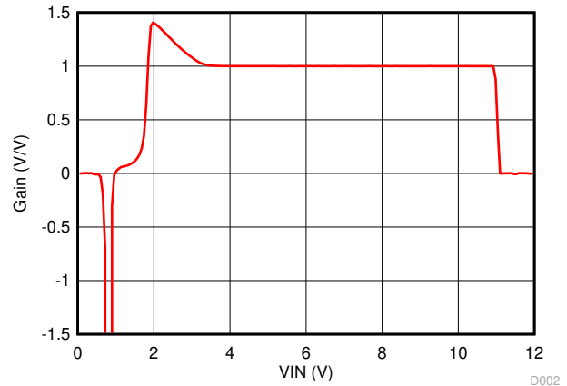
Figure 9-5. Gain vs Input Voltage
