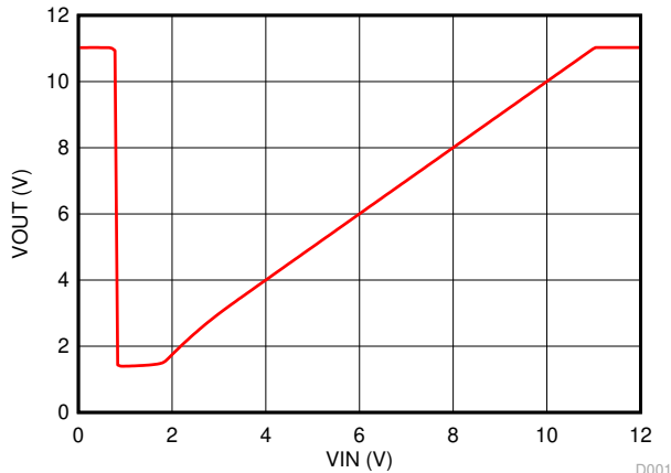
Figure 9-4. Output Voltage vs Input Voltage
