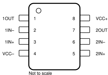
Figure 5-2. TL072x D, DDF, DGK, JG, P, PS, and PW Package 8-Pin SOIC, SOT-23 (8), VSSOP, CDIP, PDIP, SO, and TSSOP Top View
