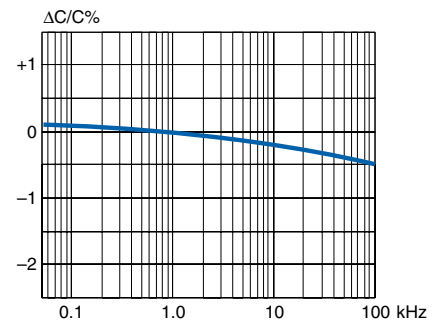
Capacitance vs. frequency (at +23^\circ C )
