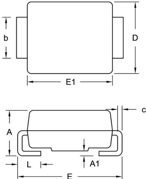
DO-214AA (SMB)
