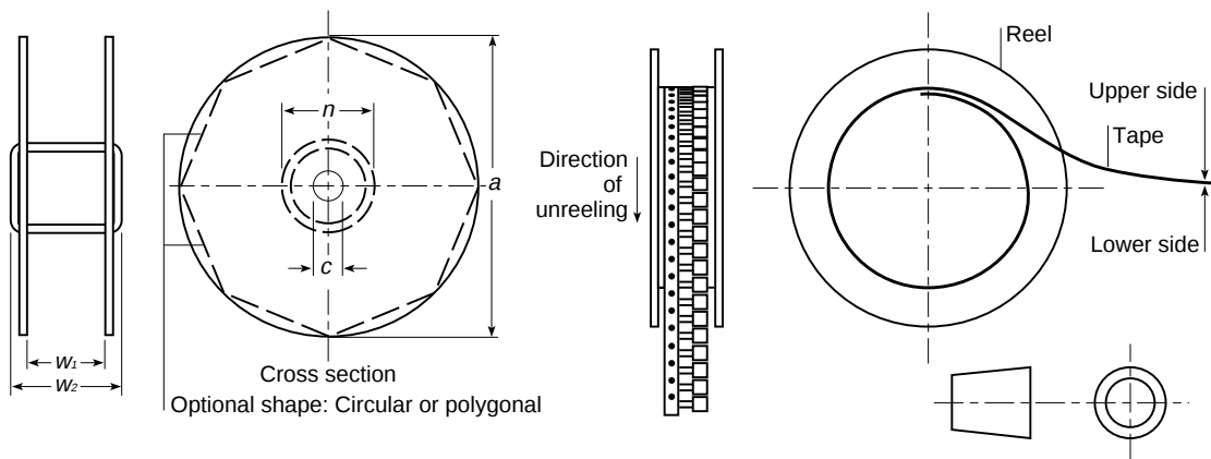
Figure R23. EIA Referenced Reel Dimensions for Radial-led Devices
