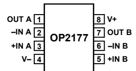
Figure 4. 8-Lead SOIC_N (R Suffix)
