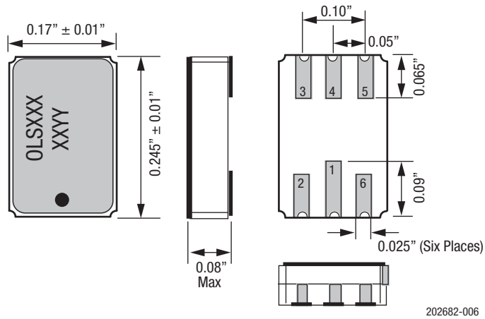
Figure 6. OLS249 Package Dimensions
