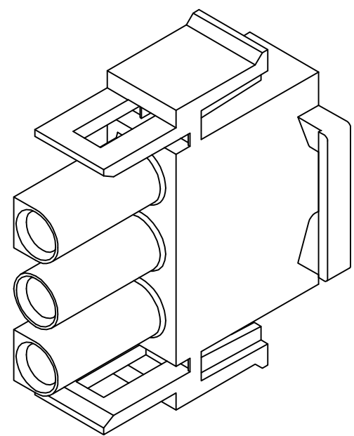
350766-4 3-DIMENSIONAL MODEL NTS
