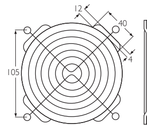
LZ30GB Welded steel guard, chromium. 4xxx and 9xxx series fans
