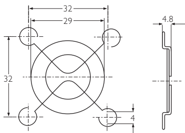
LZ29-1 Rust resistant steel wire. 4xxx series fans
