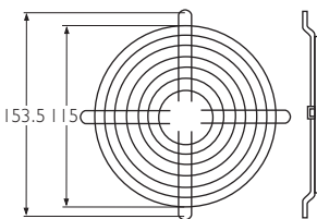
LZ30 Welded steel guard, chromium. 4xxx and 9xxx series fans
