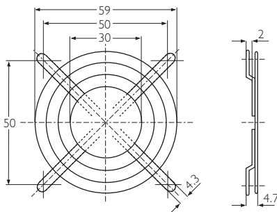
LZ28-1 Rust resistant steel wire. 6xx series fans
