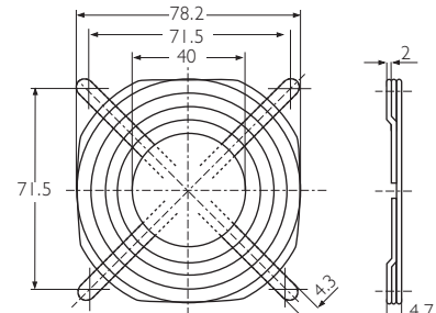
LZ32-4 Rust resistant steel wire. 8xxx series fans
