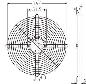
LZ37 Rust resistant steel wire. 6xxx series fans
