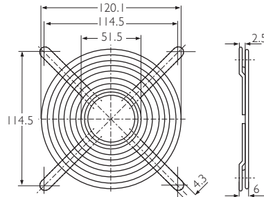
LZ35 Rust resistant steel wire. 5xxx series fans
