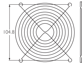
LZ30K Welded steel guard, bright nickel. 4xxx and 9xxx series fans
