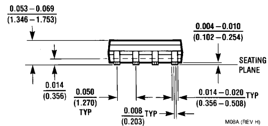
8-Pin Small Outline Package Order Number LM6142AIM, LM6142AIMX or LM6142BIM, LM6142BIMX NS Package Number M08A
