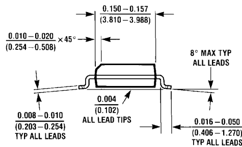
8-Pin Small Outline Package Order Number LM6142AIM, LM6142AIMX or LM6142BIM, LM6142BIMX NS Package Number M08A
