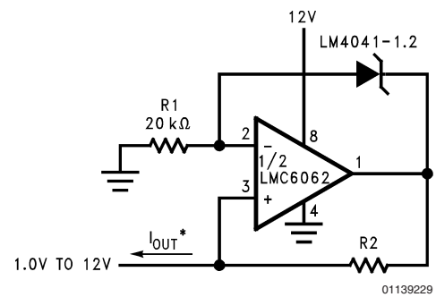
FIGURE 12. Precision Floating Current Detector
