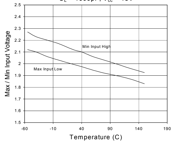
Fig. 8 Max / Min Input vs. Temperature C_L = 1000\text{pF} , V_{CC} = 18\text{V}
