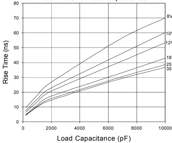
Fig. 5 Rise Times vs. Load Capacitance
