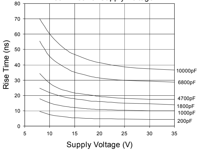
Fig. 3 Rise Times vs. Supply Voltage
