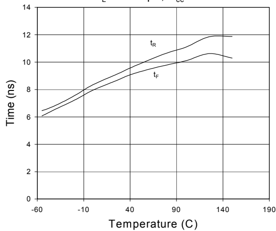
Fig. 7 Rise And Fall Times vs. Temperature C_L = 1000\text{pF} , V_{CC} = 18\text{V}
