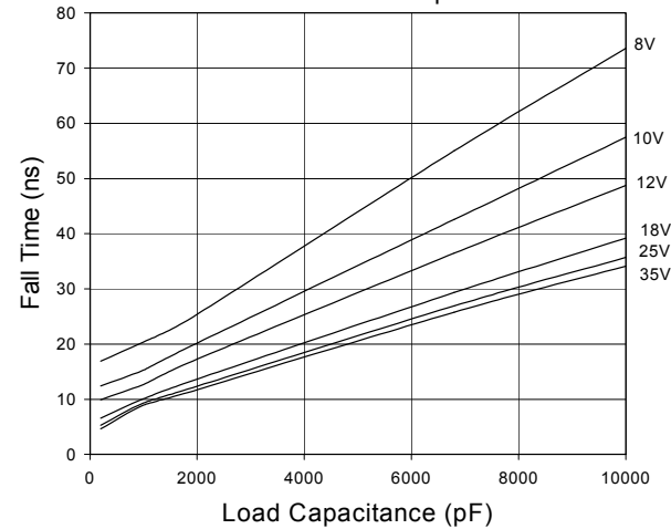
Fig. 6 Fall Times vs. Load Capacitance
