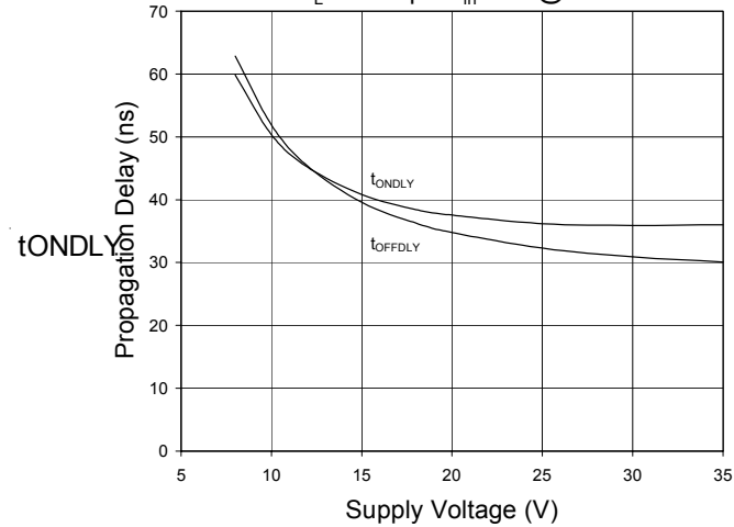
Fig. 17 Propagation Delay vs. Supply Voltage C_L = 1800pF , V_{in} = 5V@1kHz
