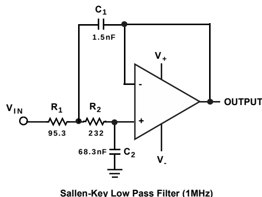
FIGURE 1. TYPICAL APPLICATION
