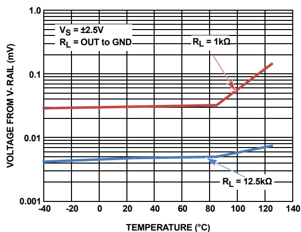
FIGURE 20. V_{OL} vs TEMPERATURE
