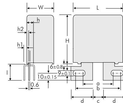
2-pin version
