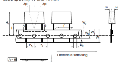
Crimped leads
