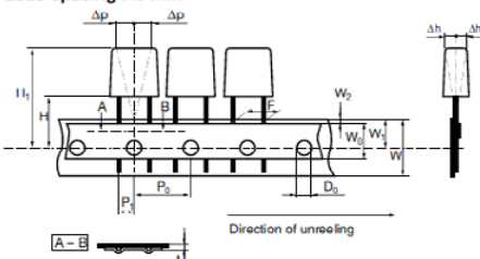
Lead spacing 22.5 and 27.5 mm
