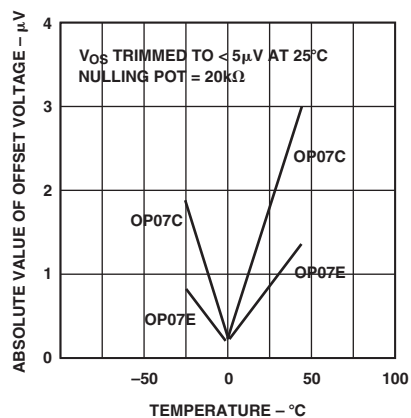
TPC 22. Trimmed Offset Voltage vs. Temperature
