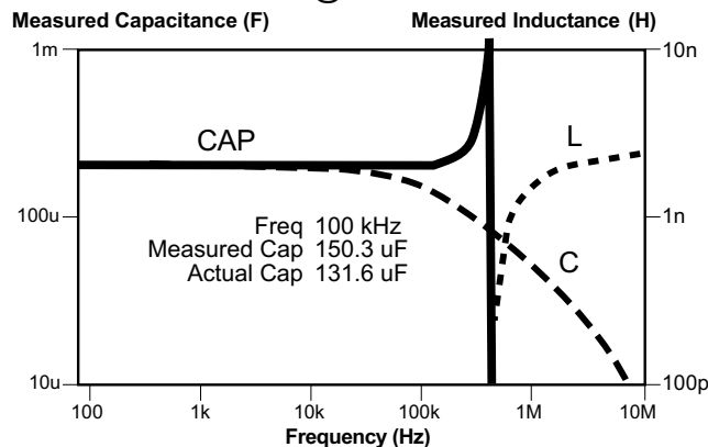
T520V157M006AS @ +25°C with 3V DC Bias
