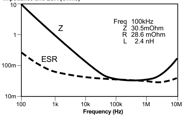
T520V157M006AS @ +25°C with 3V DC Bias
