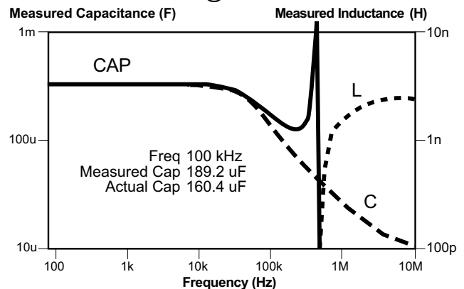
T520D337M006AS @ +25°C with 3V DC Bias
