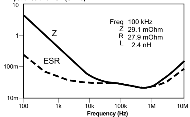
T520D337M006AS @ +25°C with 3V DC Bias
