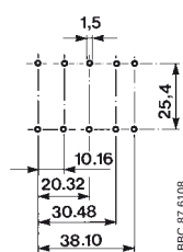
Basic devices 4-pole
