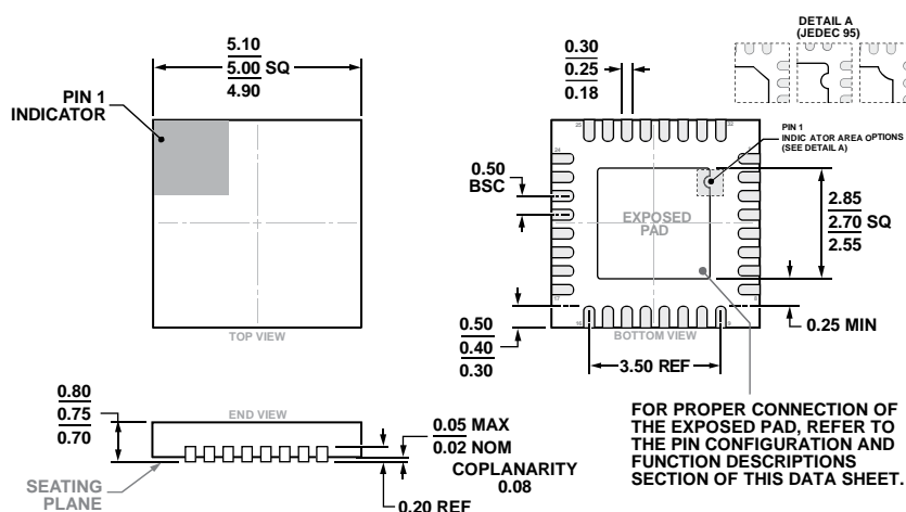
Figure 77. 32-Lead Lead Frame Chip Scale Package [LFCSP] 5 mm x 5 mm Body and 0.75 mm Package Height (CP-32-21) Dimensions shown in millimeters
