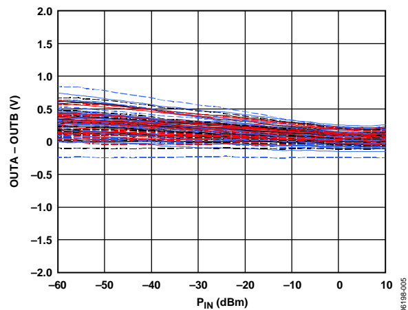
Figure 5. Distribution of [OUTA - OUTB] Voltage Difference over Temperature for 45 Devices from a Nominal Lot, Frequency = 100 MHz, ADJA , ADJB = 0.65\text{ V} , 0.7\text{ V} , Sine Wave, Single-Ended Drive
