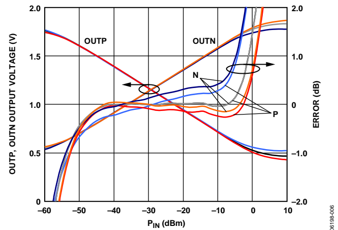
Figure 6. OUTP, OUTN Gain Error and Voltage vs. Input Amplitude at 100 MHz, Typical Device, ADJA , ADJB = 0.65\text{ V} , 0.7\text{ V} , Sine Wave, Single-Ended Drive, P_{INH} = -30\text{ dBm} , Channel A Swept
