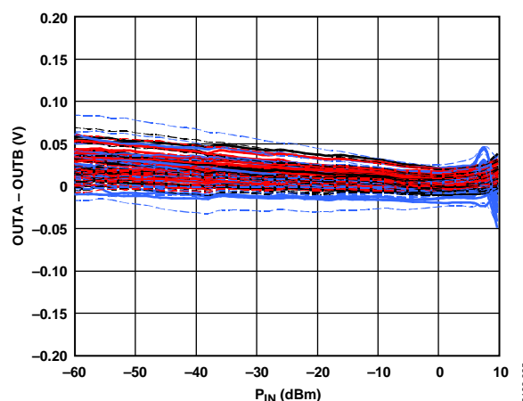
Figure 25. Distribution of [OUTA - OUTB] Voltage Difference over Temperature for 45 Devices from a Nominal Lot, Frequency = 3.6 GHz, ADJA, ADJB = 0.35 V, 0.42 V, Sine Wave, Single-Ended Drive
