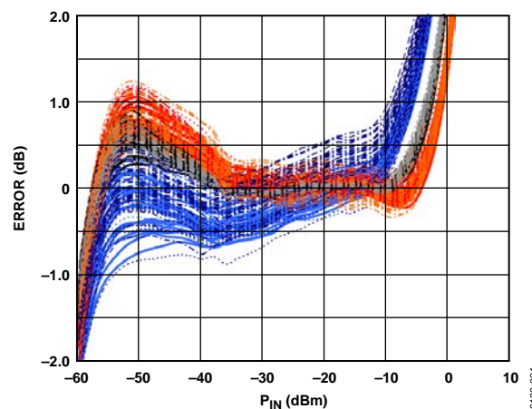
Figure 24. Distribution of OUTA, OUTB Error over Temperature After Ambient Normalization vs. Input Amplitude for 45 Devices from a Nominal Lot, Frequency = 3.6 GHz, ADJA, ADJB = 0.35 V, 0.42 V, Sine Wave, Single-Ended Drive
