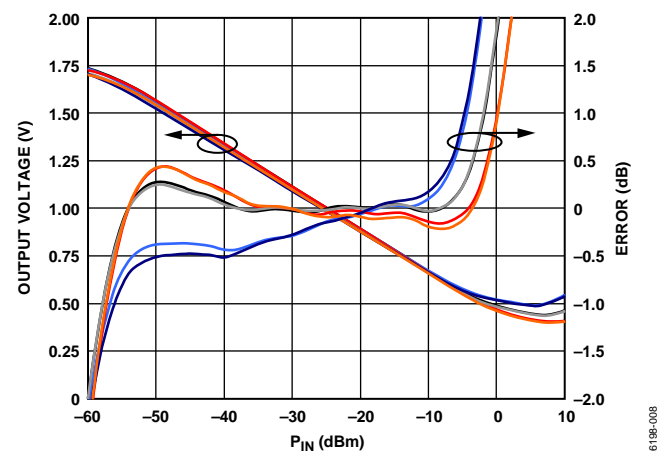
Figure 8. OUTA, OUTB Voltage and Log Conformance vs. Input Amplitude at 900 MHz, Typical Device, ADJA , ADJB = 0.6\text{ V} , 0.65\text{ V} , Sine Wave, Single-Ended Drive
