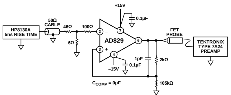
Figure 33. Follower Connection, Gain = 20
