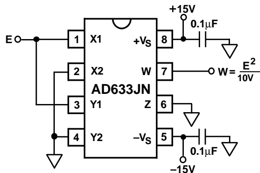
Figure 4. Connections for Squaring
