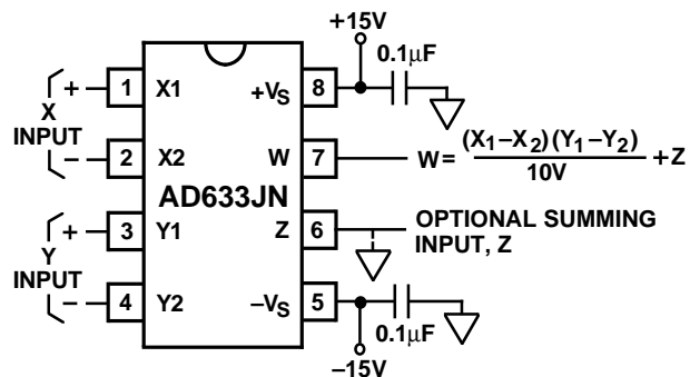
Figure 3. Basic Multiplier Connections
