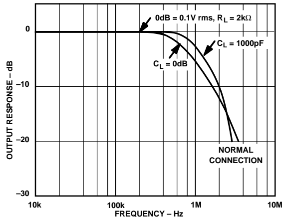
Figure 15. Frequency Response
