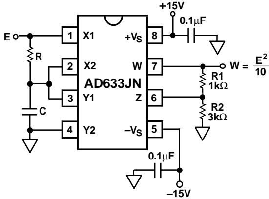
Figure 5. "Bounceless" Frequency Doubler
