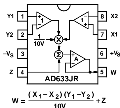
8-Pin Plastic SOIC (R) Package
