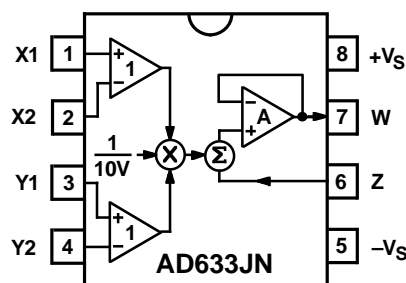
8-Pin Plastic DIP (N) Package
