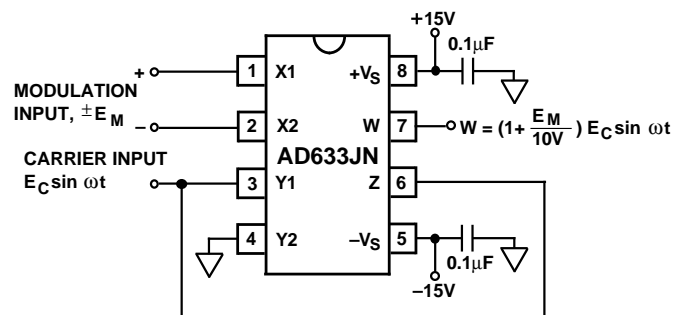
Figure 10. Linear Amplitude Modulator
