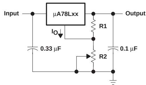
Figure 3. Adjustable-Output Regulator
