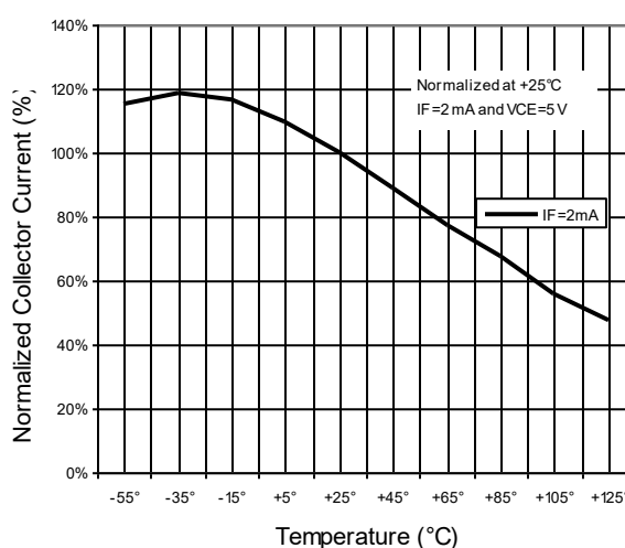
Normalized Collector Current Vs Temperature
