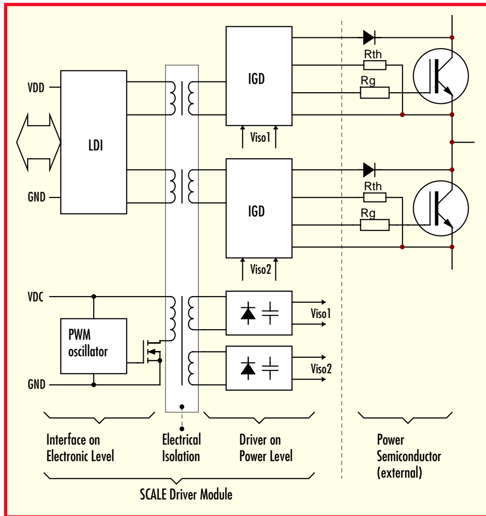
Fig. 2 Block diagram of a two-channel SCALE driver
