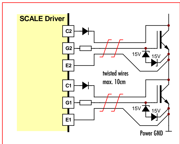
Fig. 14 Wiring driver → IGBT
