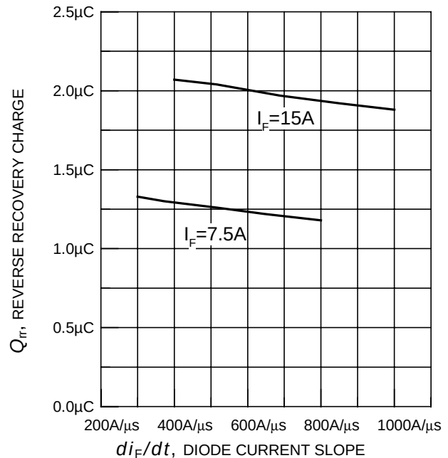
Figure 22. Typical reverse recovery charge as a function of diode current slope
