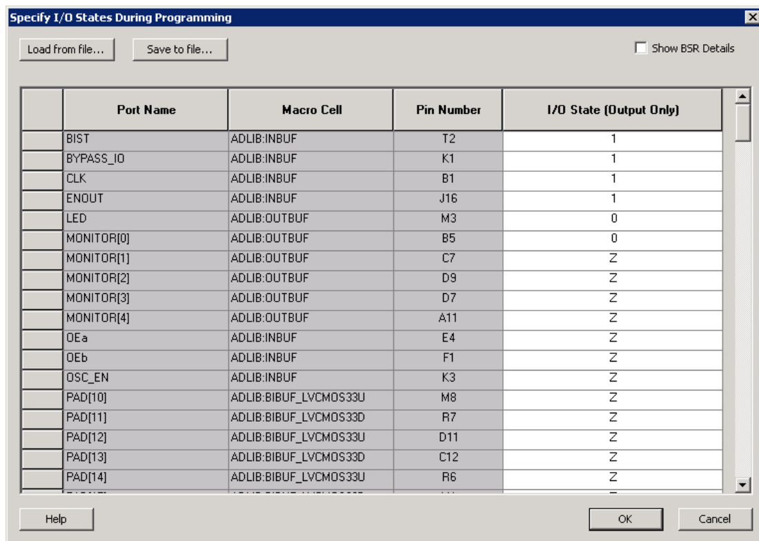
Figure 1-4 • I/O States During Programming Window
