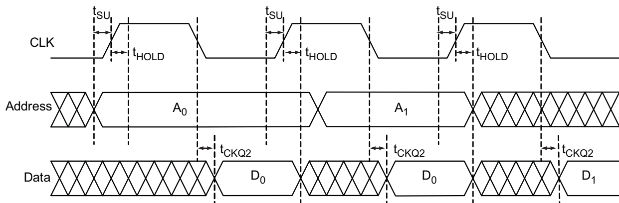
Figure 2-41 • Timing Diagram
