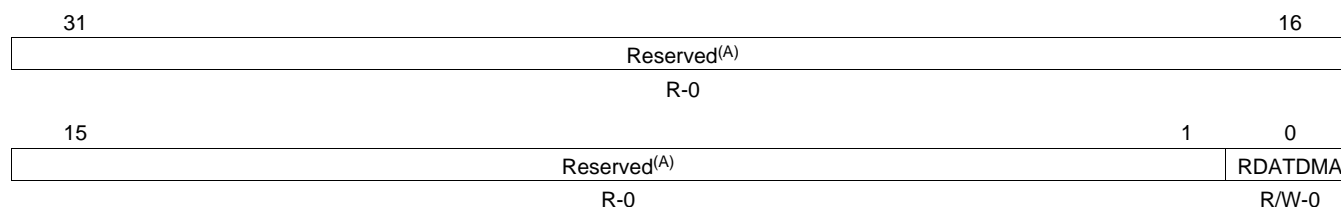
Figure 4-24. Receiver DMA Event Control Register (REVTCTL) [Offset 8Ch]
