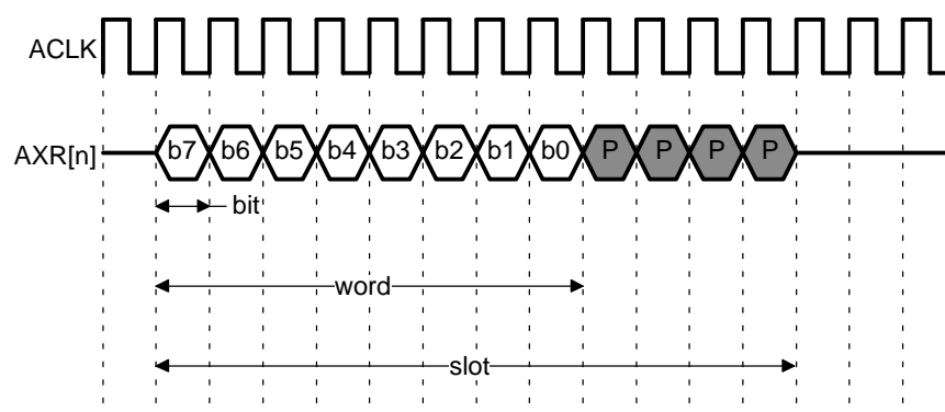
Figure 1-5. Definition of Bit, Word, and Slot
