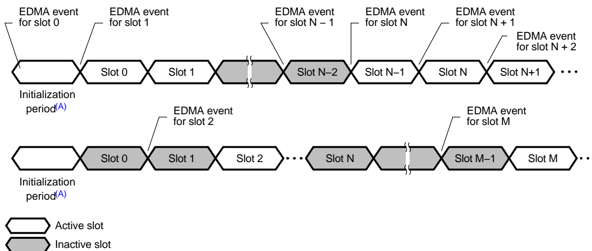
Figure 3-2. Transmit DMA Event (AXEVT) Generation in TDM Time Slots
