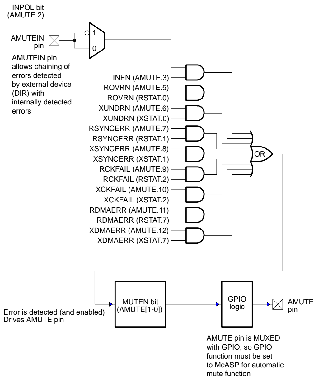
Figure 3-8. Audio Mute (AMUTE) Block Diagram
