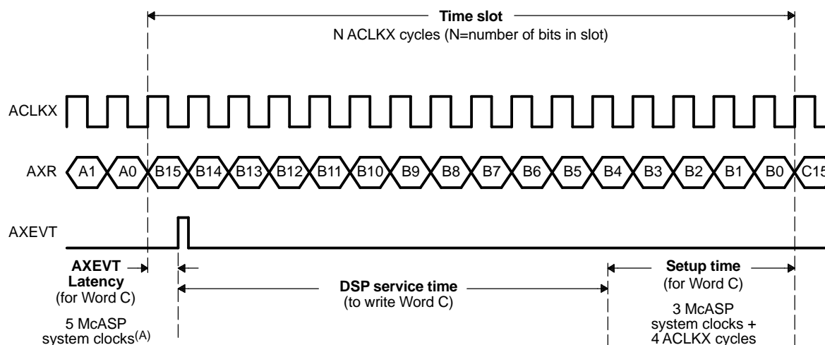
Figure 3-3. DSP Service Time Upon Transmit DMA Event (AXEVT)
