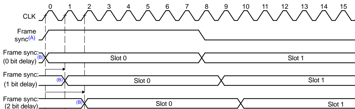
Figure 1-9. TDM Format Bit Delays from Frame Sync
