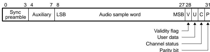
Figure 1-12. S/PDIF Subframe Format
