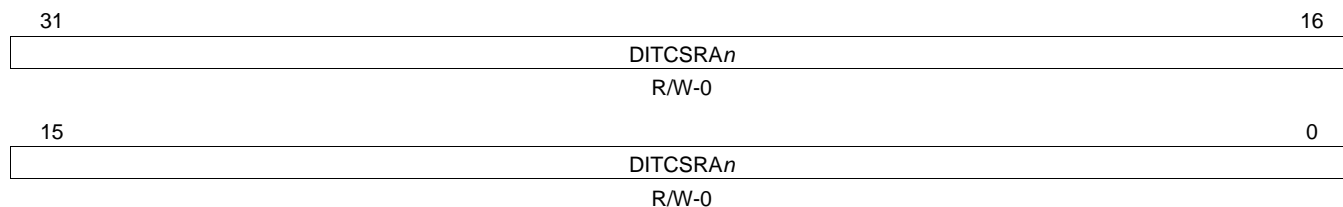
Figure 4-38. DIT Left Channel Status Registers (DITCSRA0-DITCSRA5) [Offset 100h-114h]
