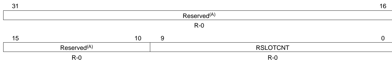
Figure 4-22. Current Receive TDM Time Slot Registers (RSLOT) [Offset 84h]
