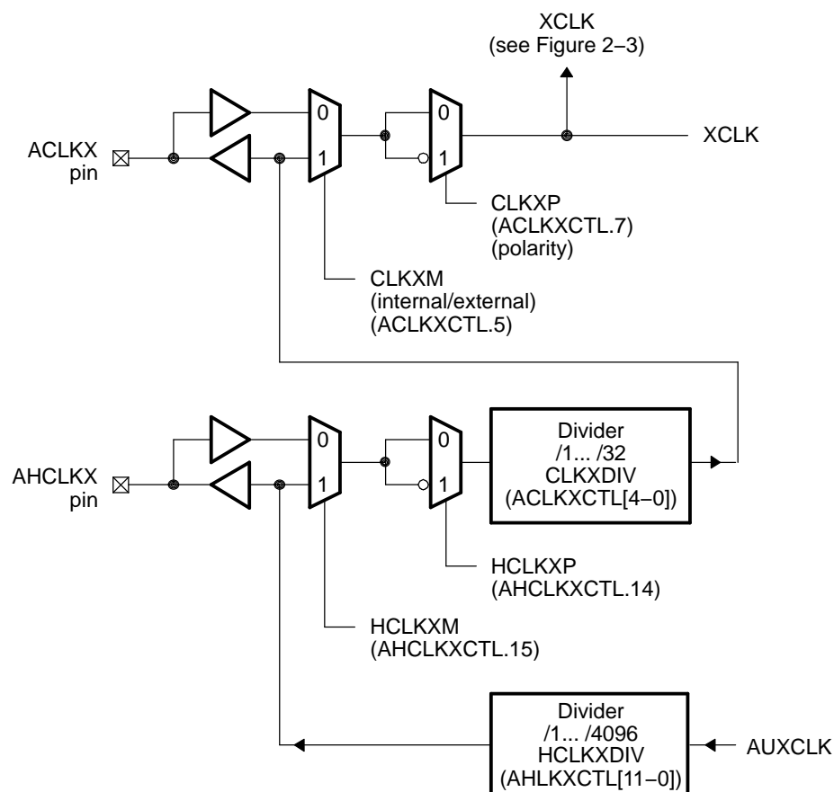
Figure 2-2. Transmit Clock Generator Block Diagram
