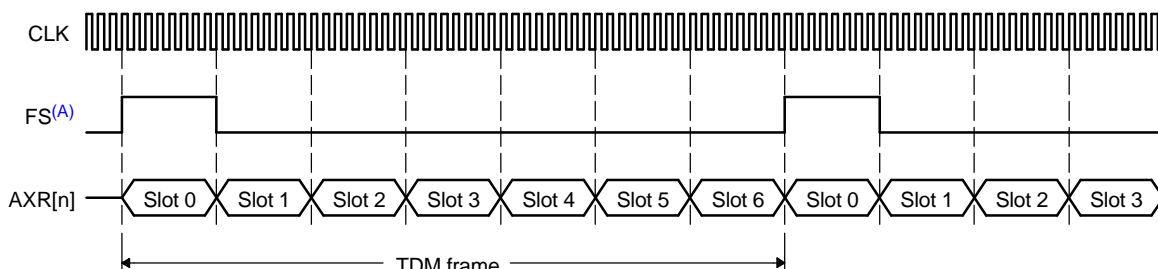
Figure 1-8. TDM Format–6 Channel TDM Example
