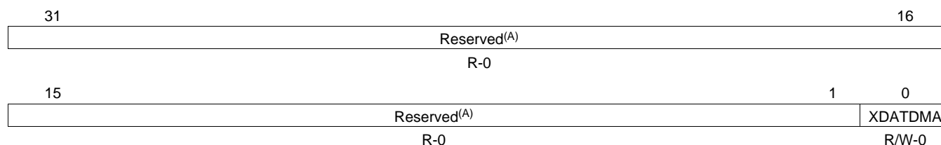
Figure 4-36. Transmitter DMA Event Control Register (XEVTCTL) [Offset CCh]
