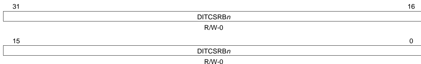
Figure 4-39. DIT Right Channel Status Registers (DITCSRB0-DITCSRB5) [Offset 118h-12Ch]
