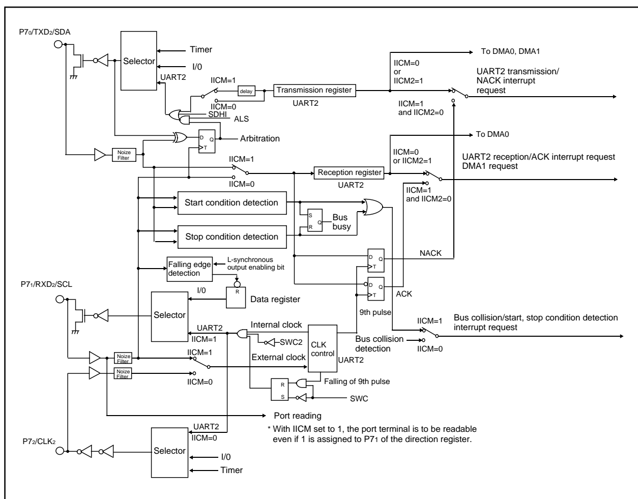
Figure 1.19.30. Functional block diagram for I²C mode
