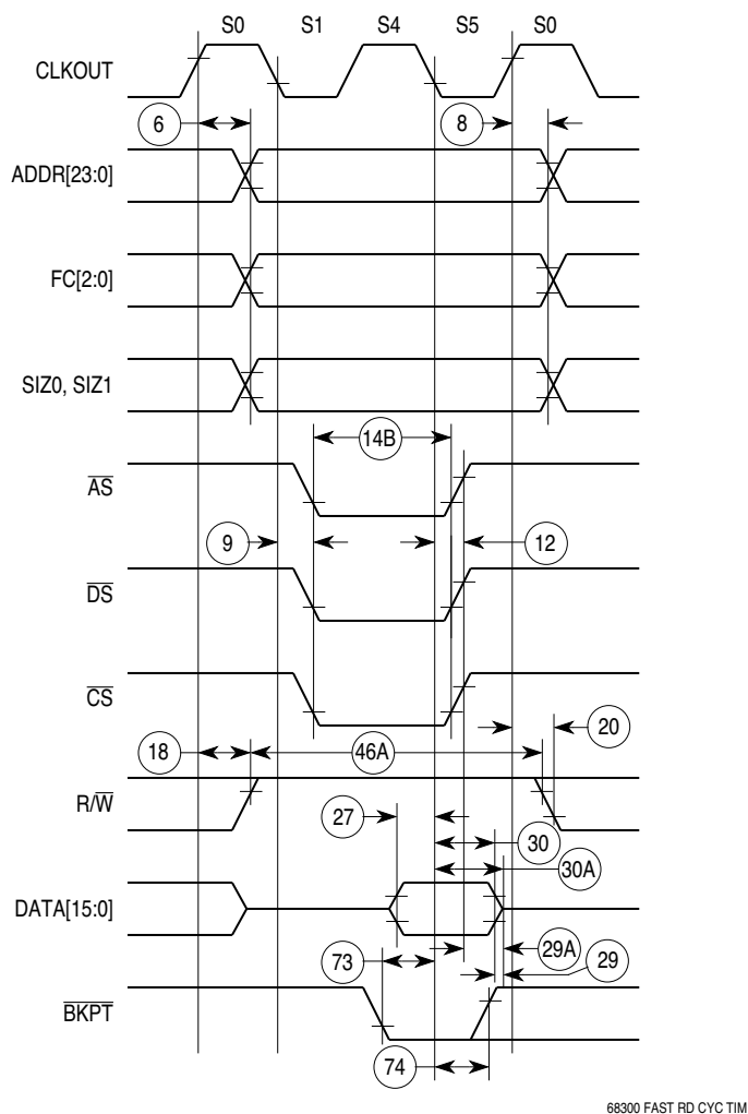
Figure A-10 Fast Termination Read Cycle Timing Diagram
