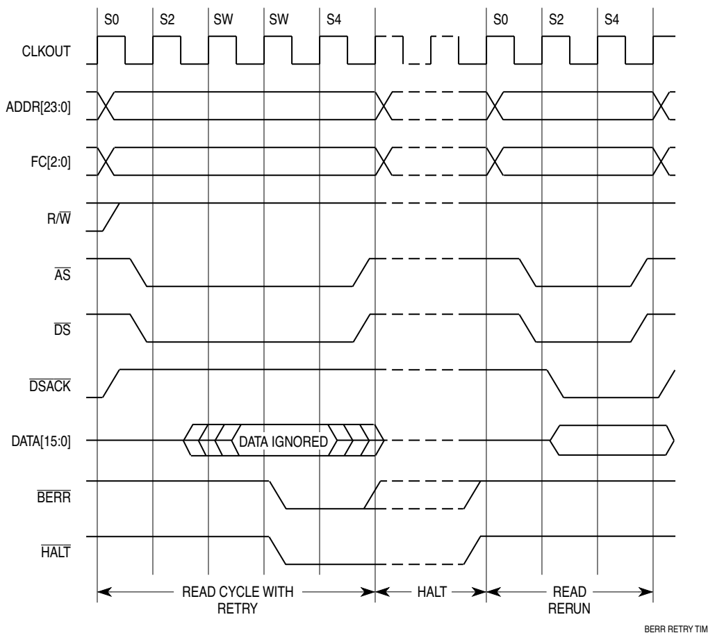
Figure 5-33 Retry Sequence
