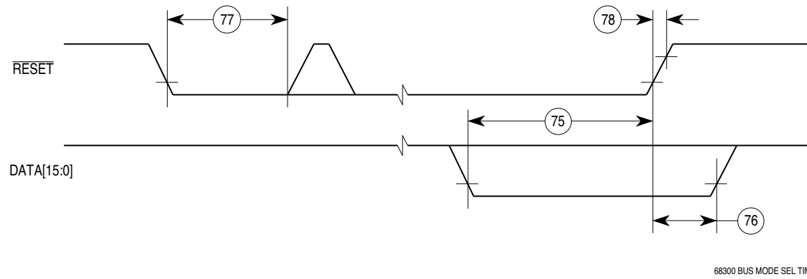
Figure A-7 Reset and Mode Select Timing Diagram
