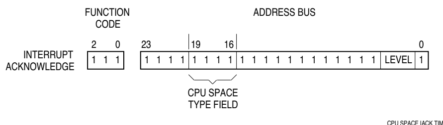
Figure 7-4 CPU Space Encoding for Interrupt-Acknowledge Cycles
