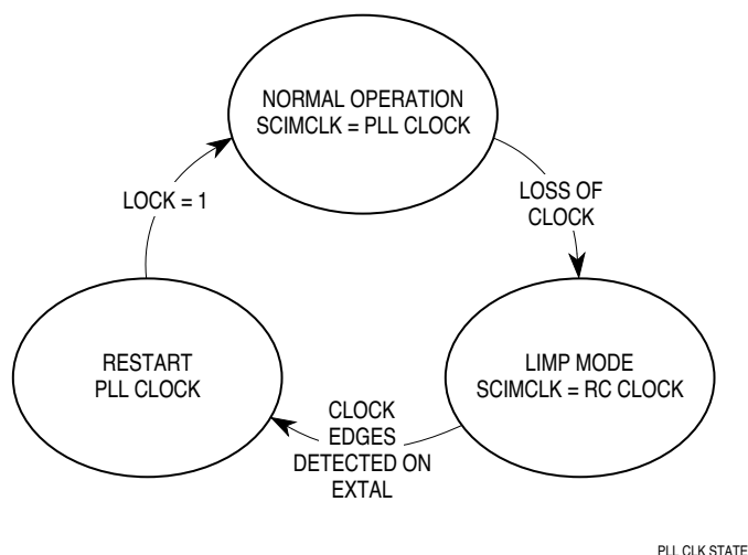
Figure 4-5 Loss of Reference Frequency
