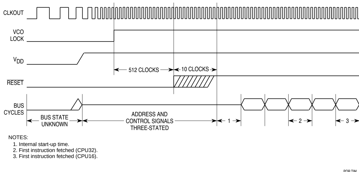
Figure 8-3 Power-On Reset Timing
