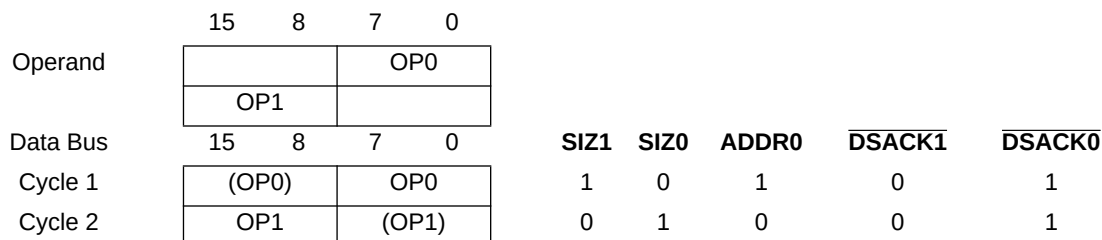
Figure 5-14 Word Operand to 16-Bit Port, Misaligned
