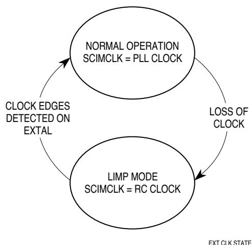
Figure 4-6 Loss of External Clock Signal
