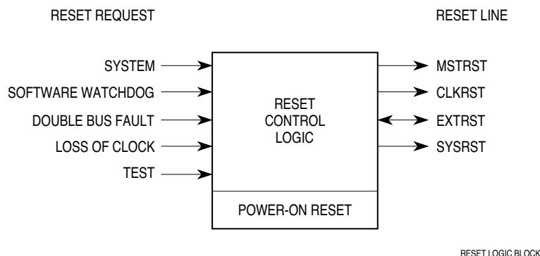
Figure 8-1 Reset Block Diagram
