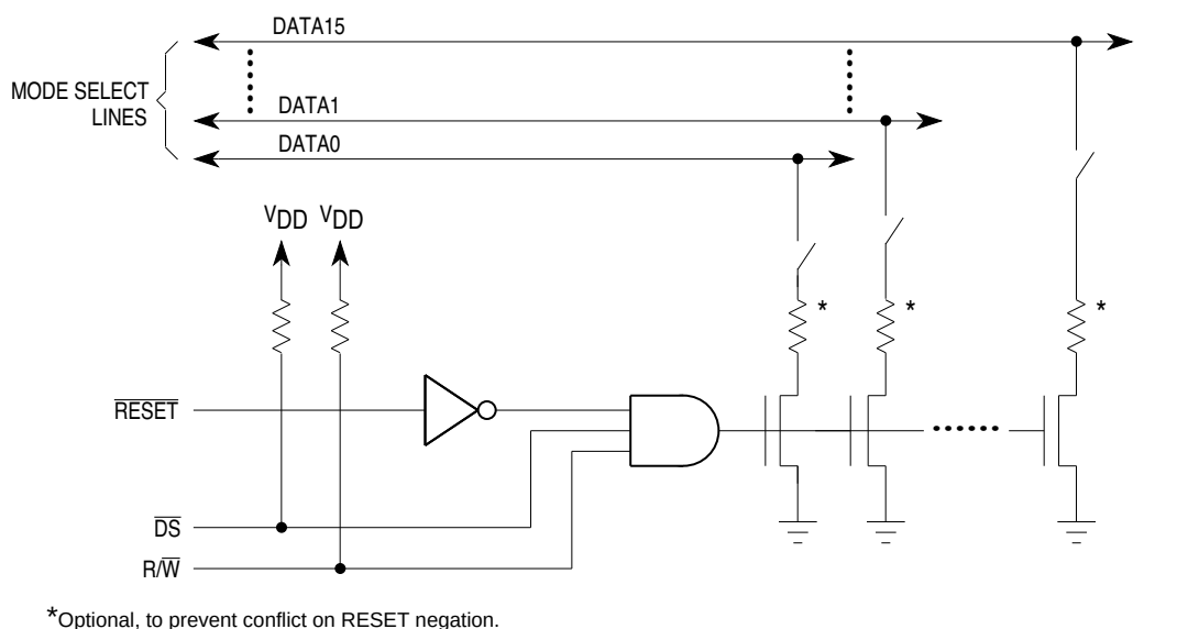
Figure 8-4 Data Bus Signal Conditioning
