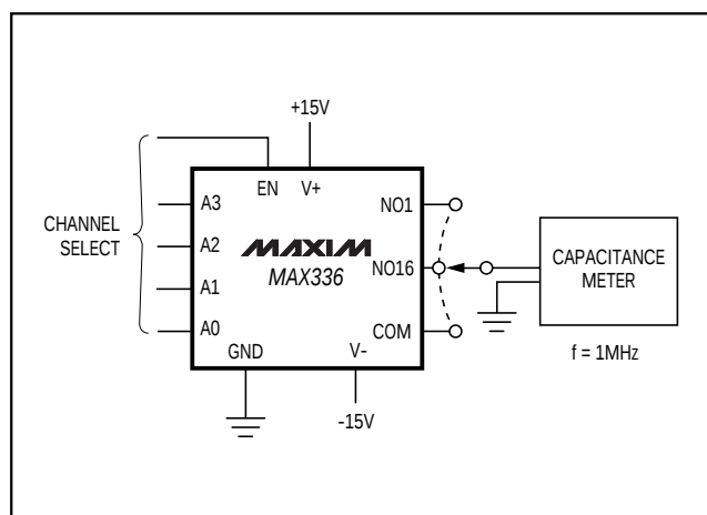
Figure 8. NO/COM Capacitance
