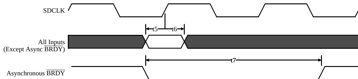
Figure 6. Memory Interface Input Timing Diagram
