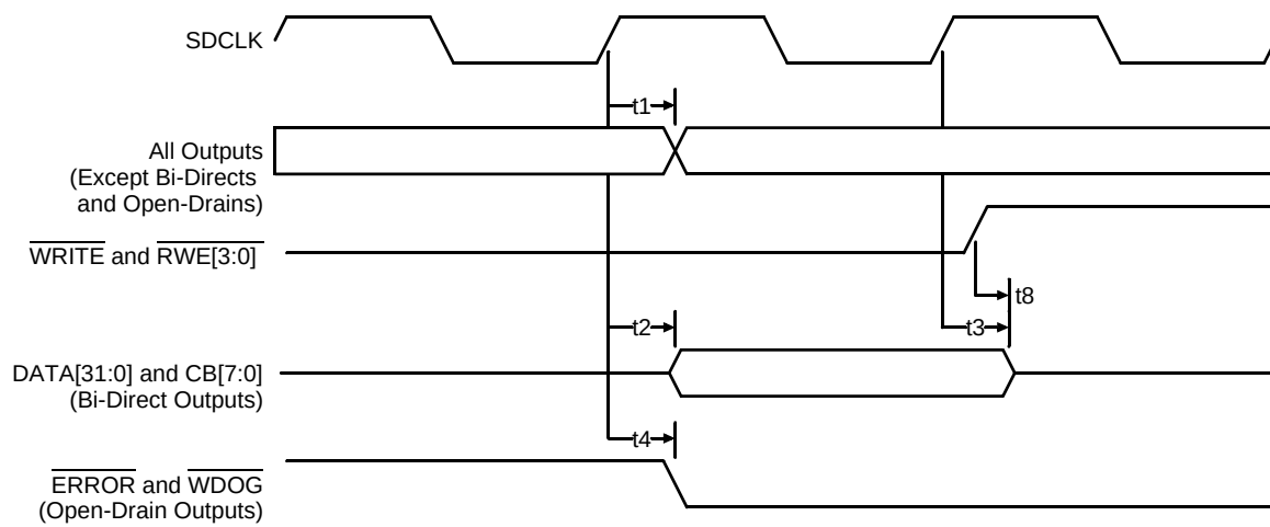
Figure 5. Memory Interface, \overline{\text{ERROR}} , and \overline{\text{WDOG}} Output Timing Diagram
